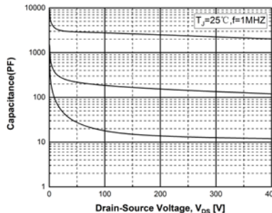
Fig. 8. Characteristics vs. Drain-to-Source Voltage
