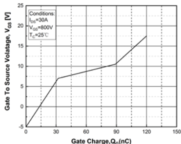
Fig. 7. Gate Charge Characteristics
