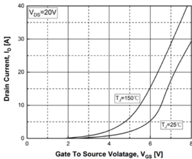
Fig. 5. Transfer Characteristics
