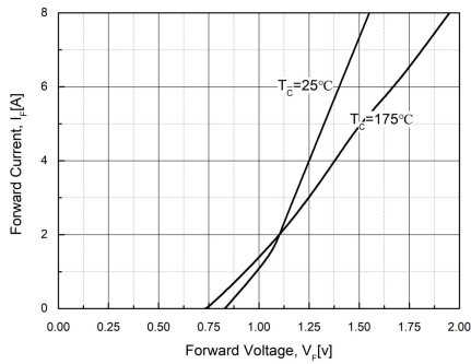
Fig. 1. Typical Characteristics: V_F vs. I_F
