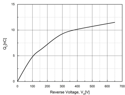
Fig. 3. Typical Characteristics: V_R vs. Q_C
