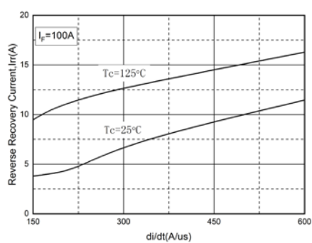
Fig. 4. Typical Reverse Recovery Current vs. di/dt
