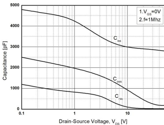
Fig. 5. Capacitance Characteristics
