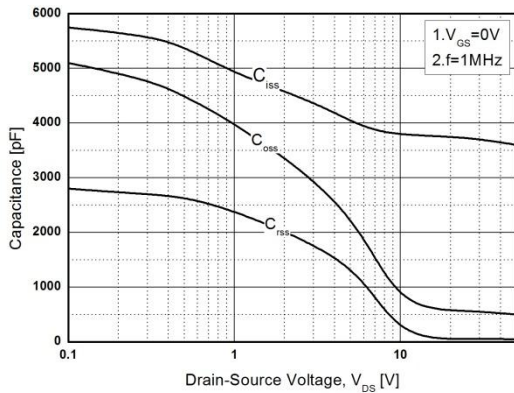
Fig. 5. Capacitance Characteristics
