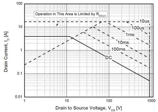
Fig. 10. Maximum Safe Operating Area-SQPF4N90
