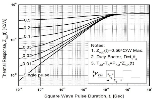
Fig. 11. Transient Thermal Response Curve
