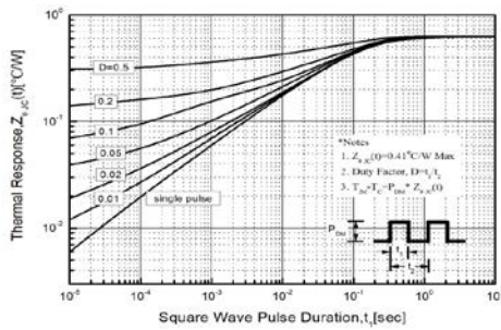
Fig. 11. Transient Thermal Response Curve
