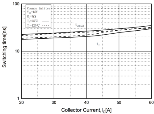
Fig. 9. Turn-on Characteristics vs. I_C
