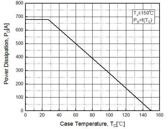
Fig. 8. Power Dissipation vs. T_C
