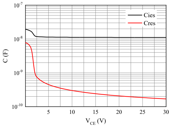
Fig 5. Capacitance characteristic
