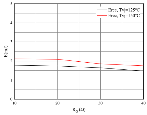
Fig 8. Switching losses of Diode I_F=30A , V_{CE}=600V
