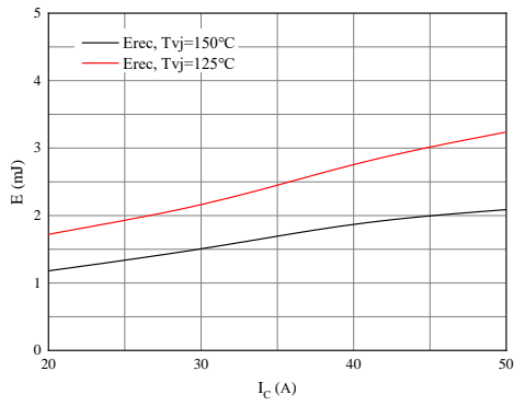
Fig 7. Switching losses of Diode R_{Gon}=10 \Omega , V_{CE}=600V
