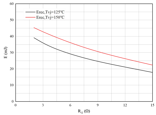
Fig 8. Switching losses of Diode I C =450A, V CE =600V
