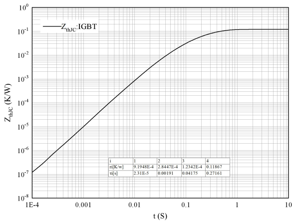
Fig 11. Transient thermal impedance IGBT, Inverter Z thJC =f(t)
