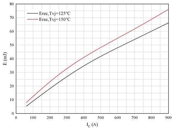
Fig 7. Switching losses of Diode R Gon =2.0Ω, V CE =600V
