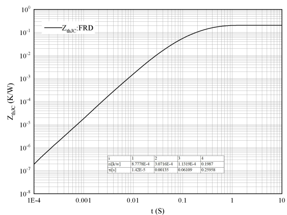
Fig 12. Transient thermal impedance FRD, Inverter Z thJC =f(t)
