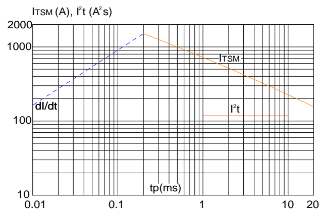
Fig.5 : Non-repetitive surge peak on-state current for a sinusoidal pulse with width t_p < 20\text{ms} and corresponding value of I t ( dI/dt < 50\text{A}/\mu\text{s} )
