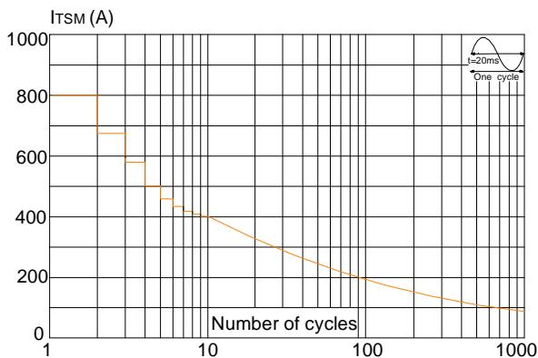
Fig.5 : Non-repetitive surge peak on-state current for a sinusoidal pulse with width t_p < 20\text{ms} and corresponding value of I_t t ( dI/dt < 100\text{A}/\mu\text{s} )
