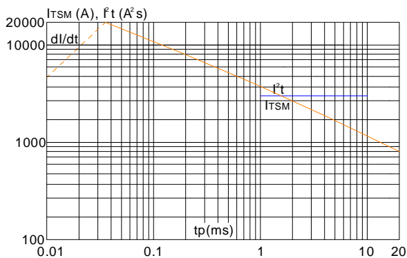
Fig.5 : Non-repetitive surge peak on-state current for a sinusoidal pulse with width t_p < 20\text{ms} and corresponding value of I_t t ( dI/dt < 100\text{A}/\mu\text{s} )
