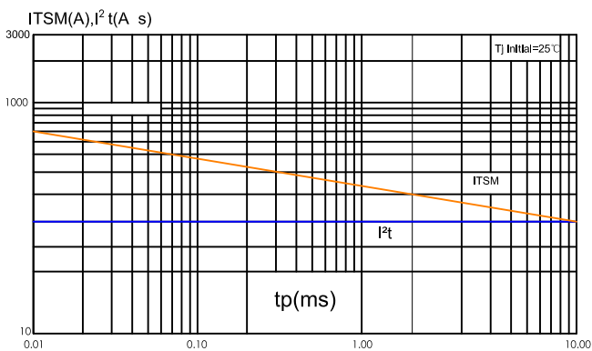
Fig.5 : Non-repetitive surge peak on-state current for a sinusoidal pulse with width t_p < 20\text{ms} and corresponding value of I t ( dI/dt < 100\text{A}/\mu\text{s} )
