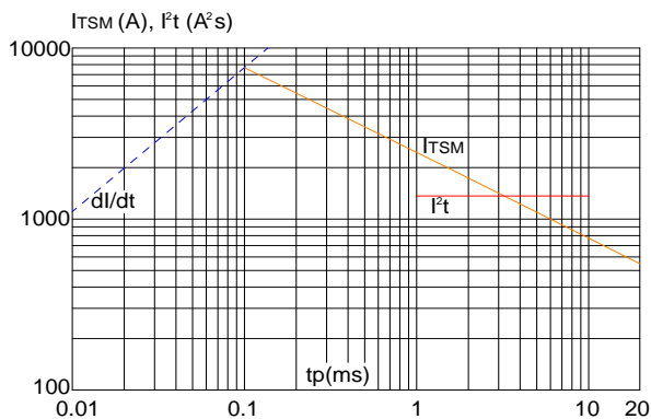
Fig.5 : Non-repetitive surge peak on-state current for a sinusoidal pulse with width t_p < 20ms and corresponding value of I_t ( dI/dt < 100A/\mu s )
