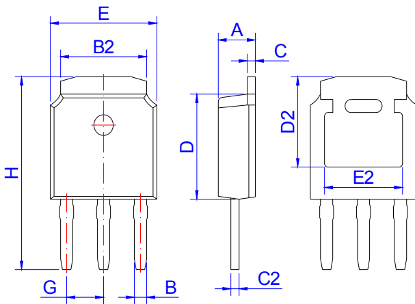
TO-251
