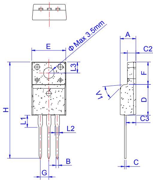
TO-220F
